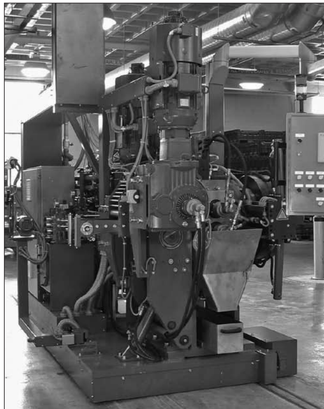
LMI strains in-line an average of 1.5 metric tons (3,300 pounds) of rubber per hour using the roll-ex ® gear extruder.
